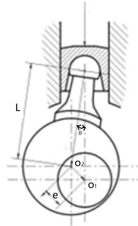
Schenatic diagram
