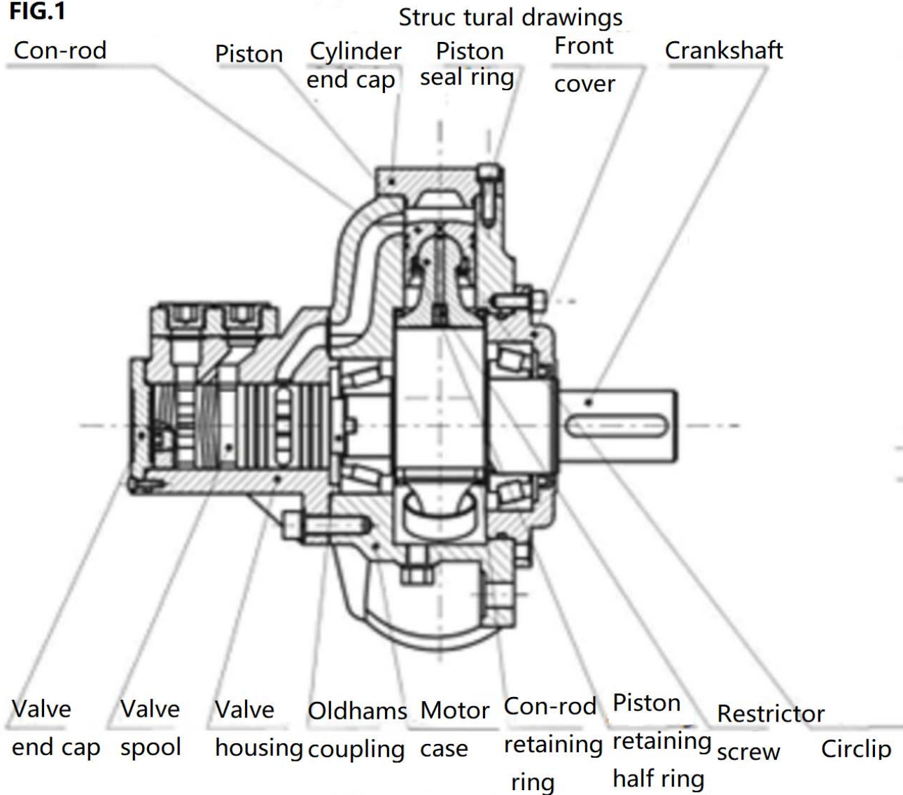
Schenatic diagram
